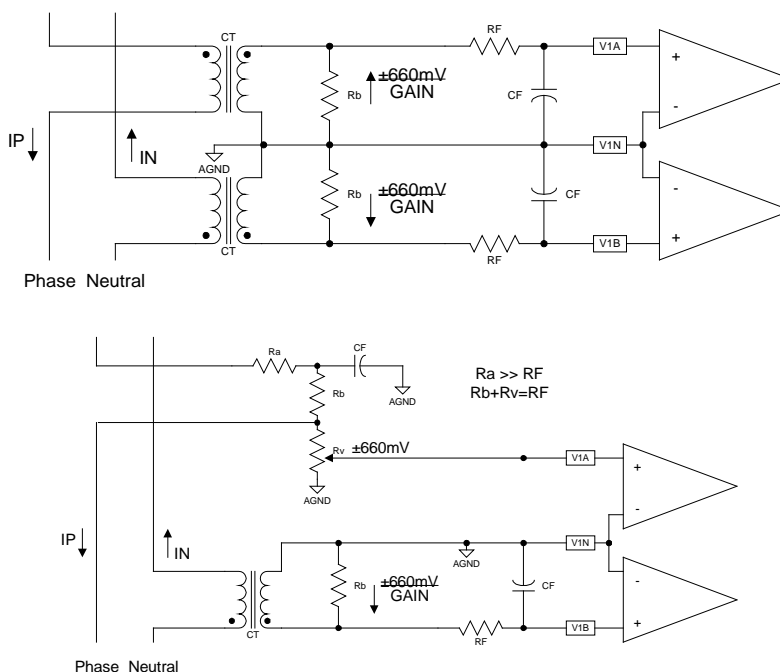
Figure 7. Typical Connections for Current Channels
