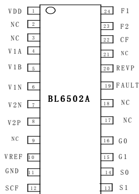
DIP/SSOP 24
