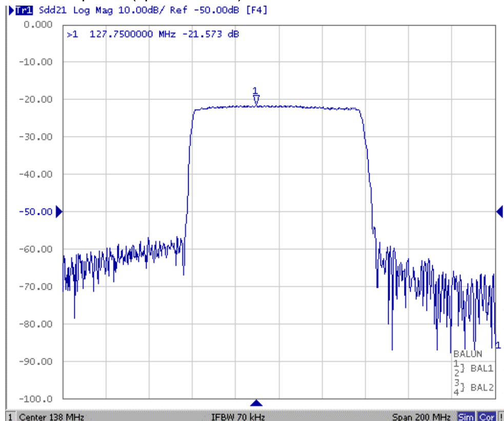
Fig1. Horizontal: 20MHz/Div Vertical: 10dB/Div
