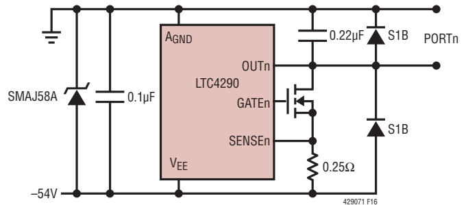
Figure 16. LTC4290 Discharge Protection
