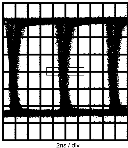
Figure 3-5. MLT-3 Total Jitter=1.9ns Pk-Pk
