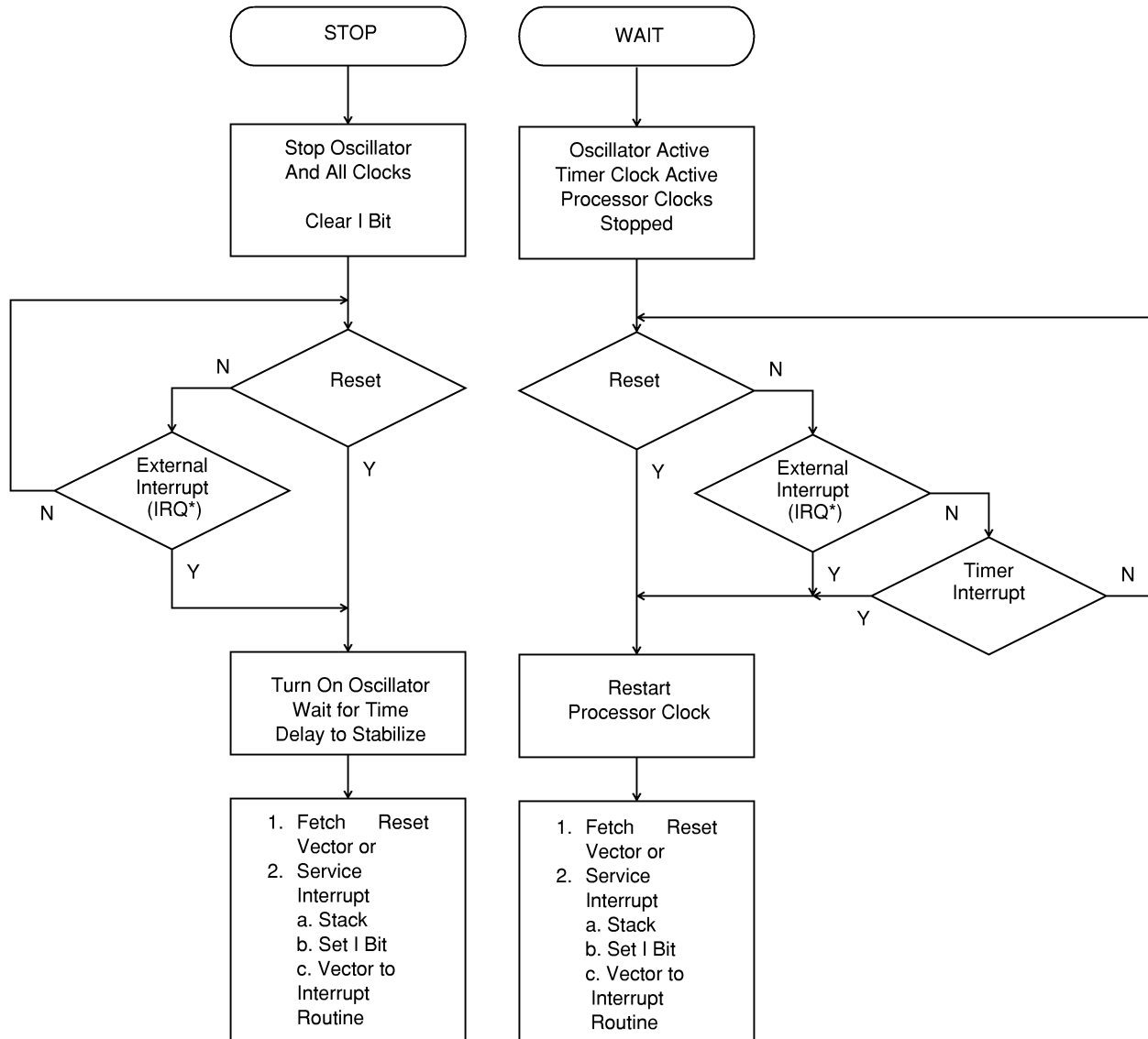
Figure 4-5: STOP/WAIT Flowcharts
