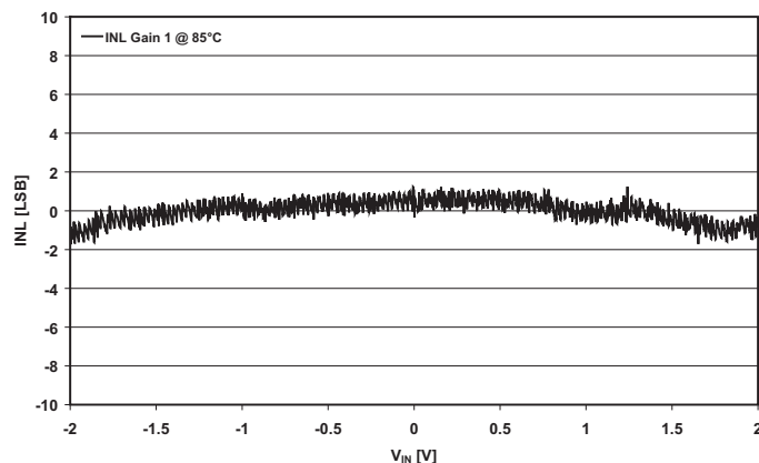
Figure 37. INL 85°C
