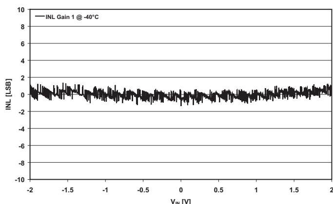
Figure 35. INL -40°C
