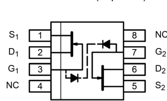
P-DIP / SOIC (Top View)
