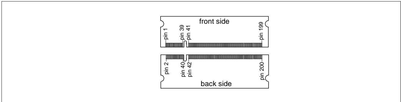
Figure 1 Pin Configuration
