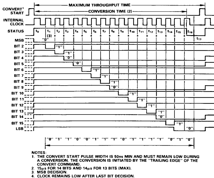
Figure 6. Timing Diagram (Binary Code 0110011101111010)
