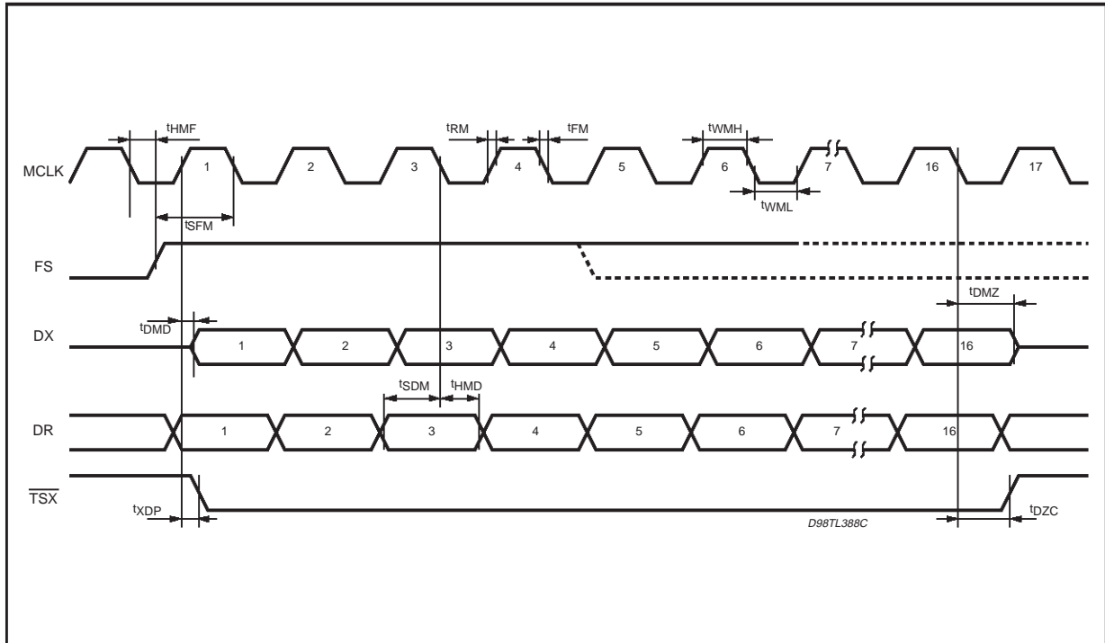
Figure 6c. MCU Mode Frame Sync. Timing.
