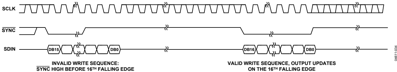
Figure 35. \overline{SYNC} Interrupt Facility
