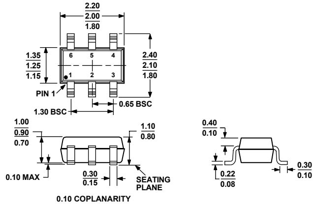
COMPLIANT TO JEDEC STANDARDS MO-203-AB Figure 45. 6-Lead Thin Shrink Small Outline Transistor Package [SC70] (KS-6) Dimensions shown in millimeters
