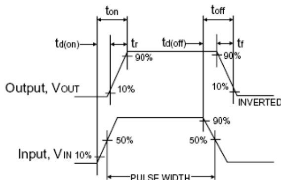
Switchin Waveforms
