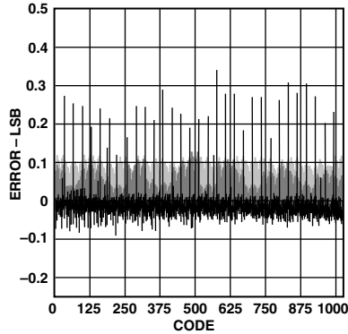
Figure 34. Typical DNL
