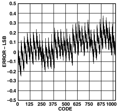
Figure 33. Typical INL
