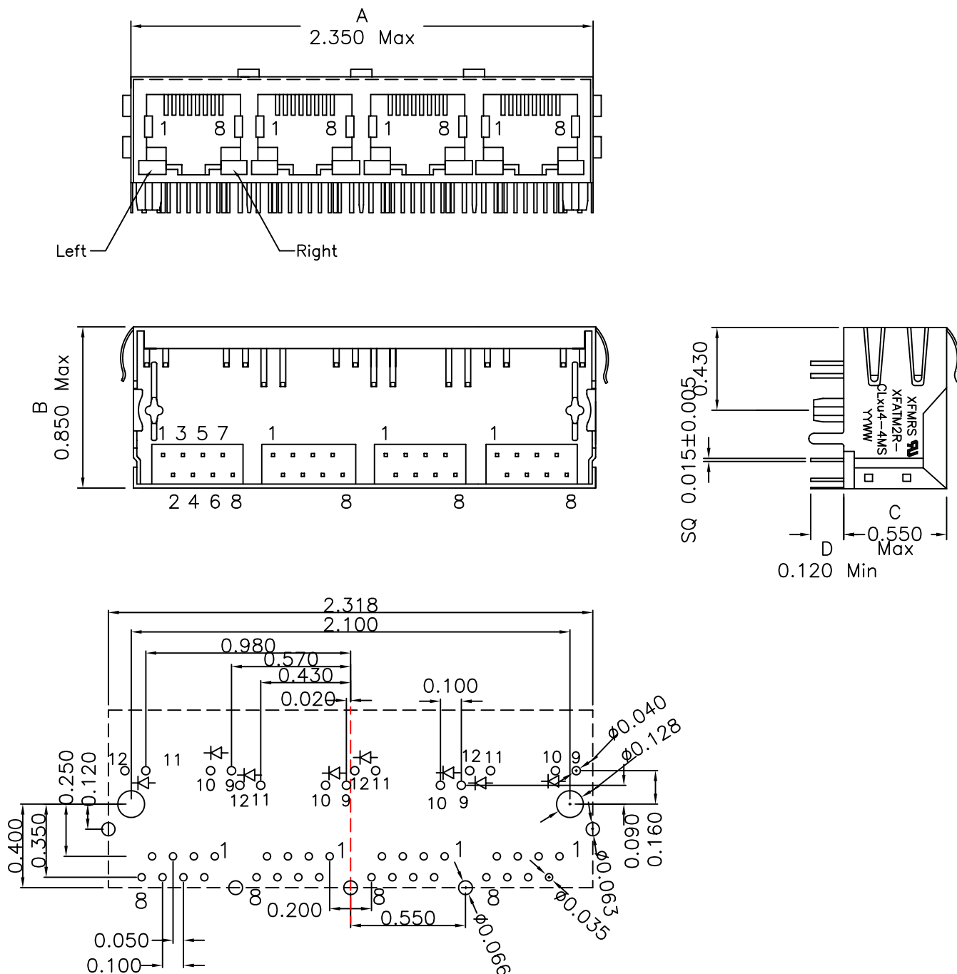
SUGGESTED MOUNTING PATTERN
