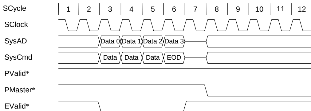
Figure 6.3.20 Block Read Response, System Interface Already In Slave State
