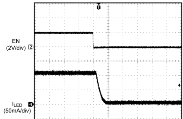
ON to Standby
