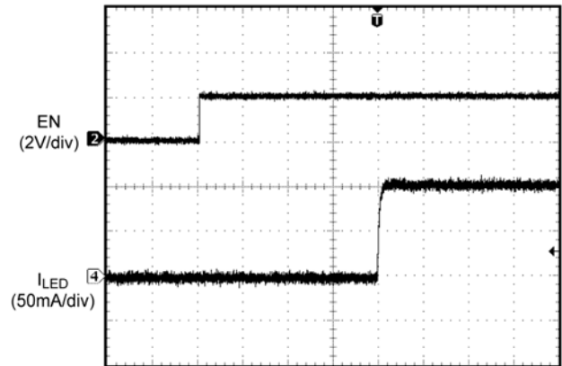
Shutdown to ON
