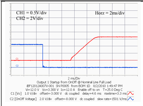
I_o=1.8V Typical startup characteristic from on/off at light load. Upper trace - output voltage, lower trace – on/off signal
