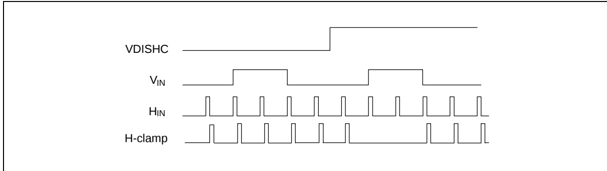
Figure 16. Disable H-clamp output
