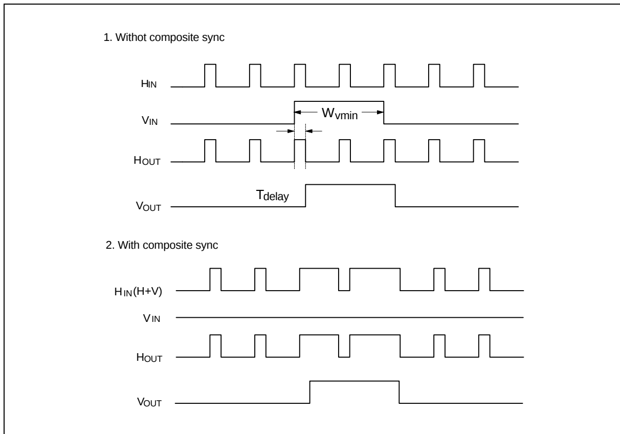
Figure 12. Vsync separator output (when DUMMYEN = 0, ENVS = 1)
