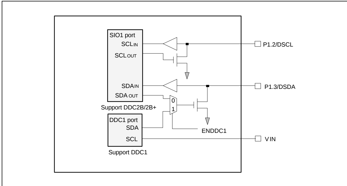
Figure 5. DDC port
