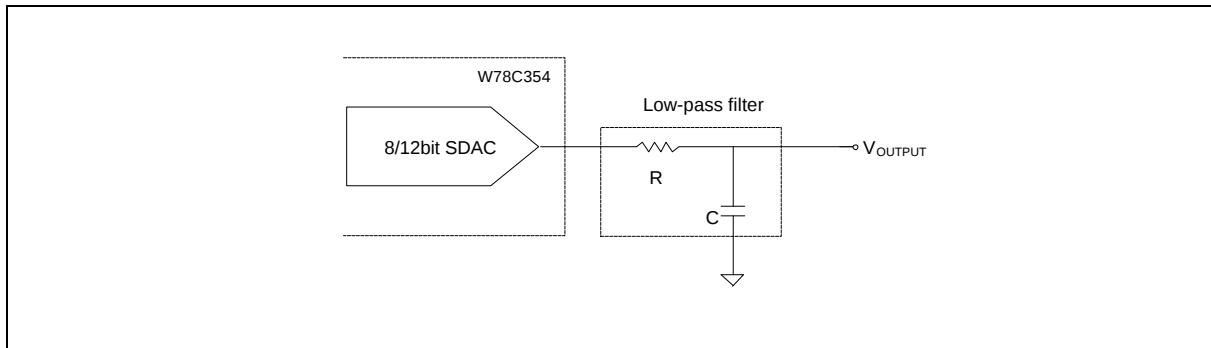
Figure 8. SDAC application circuit (where T = RC , V_{\text{OUTPUT}} = V_{\text{CC}} \times n/255 , if T \gg T_{\text{PWM}} )
