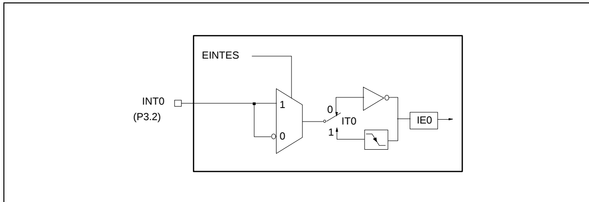
Figure 7. External interrupt 0
