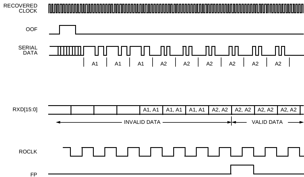
Figure 11. Frame and Byte Detection
