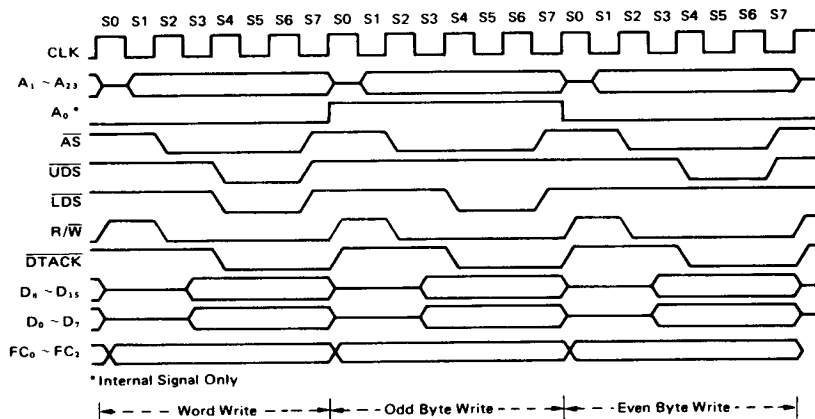
Figure 21 Word and Byte Write Cycle Timing Diagram
