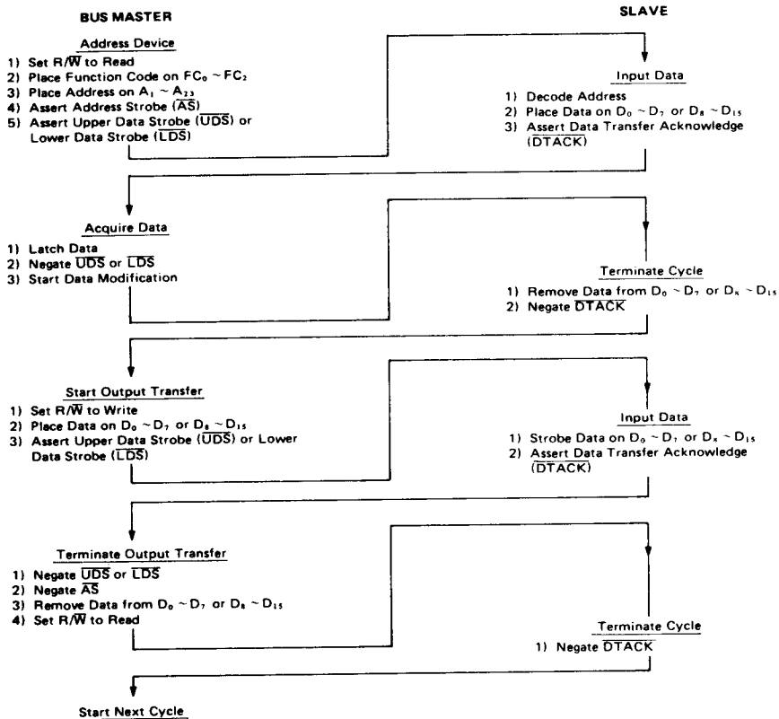
Figure 22 Read-Modify-Write Cycle Flow Chart
