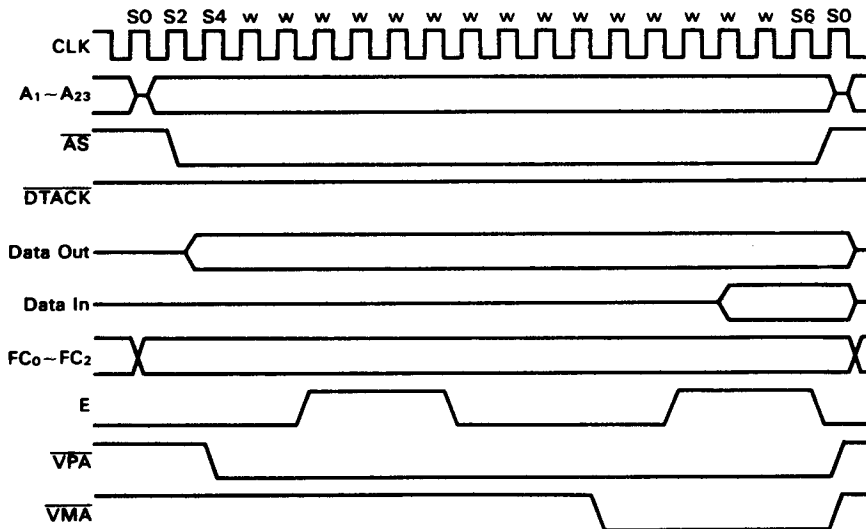
Figure 50 68000 to HD6800 Peripheral Timing—Worst Case
