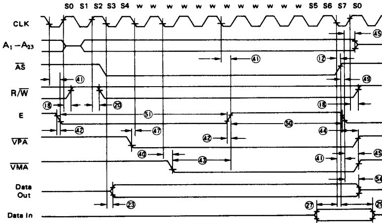
Figure 5. HD6800 Timing—Best Case
