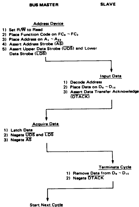
Figure 15 Word Read Cycle Flow Chart
