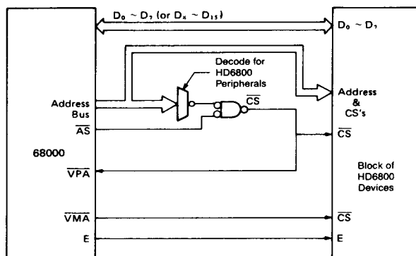
Figure 47 Connection of HD6800 Peripherals
