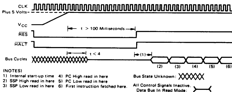
Figure 35 Reset Operation Timing Diagram
