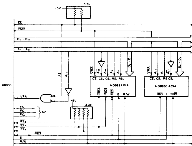
Figure 52 HD6800 Interface—Example 1
