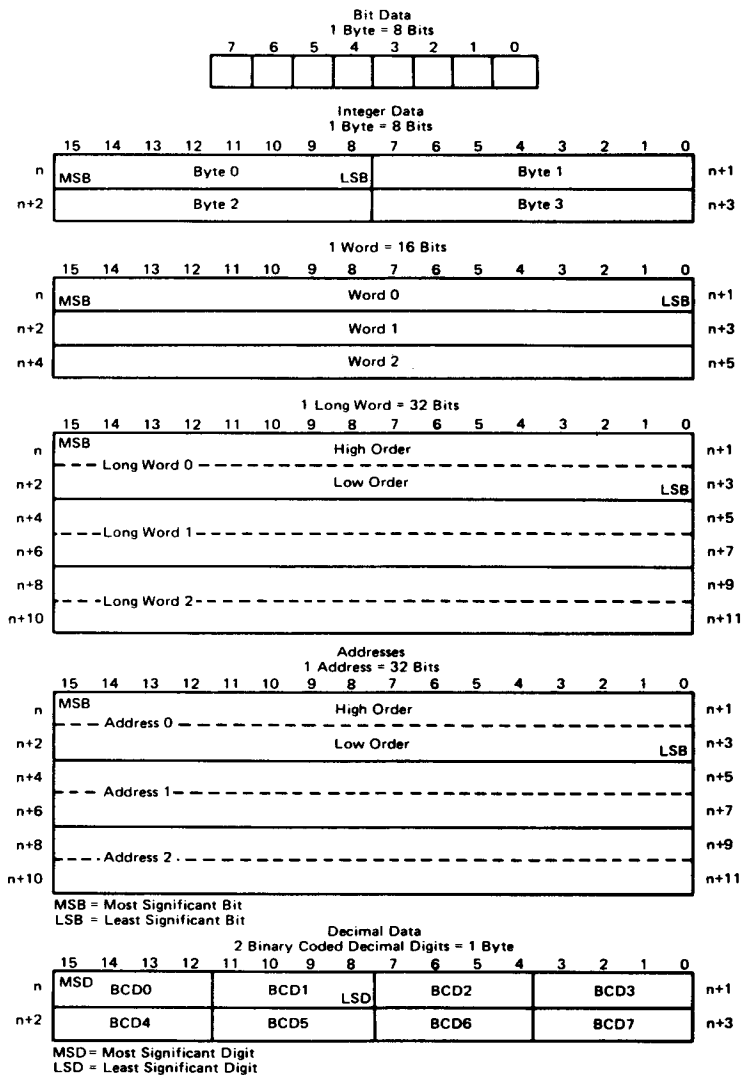
Figure 11 Data Organization in Memory
