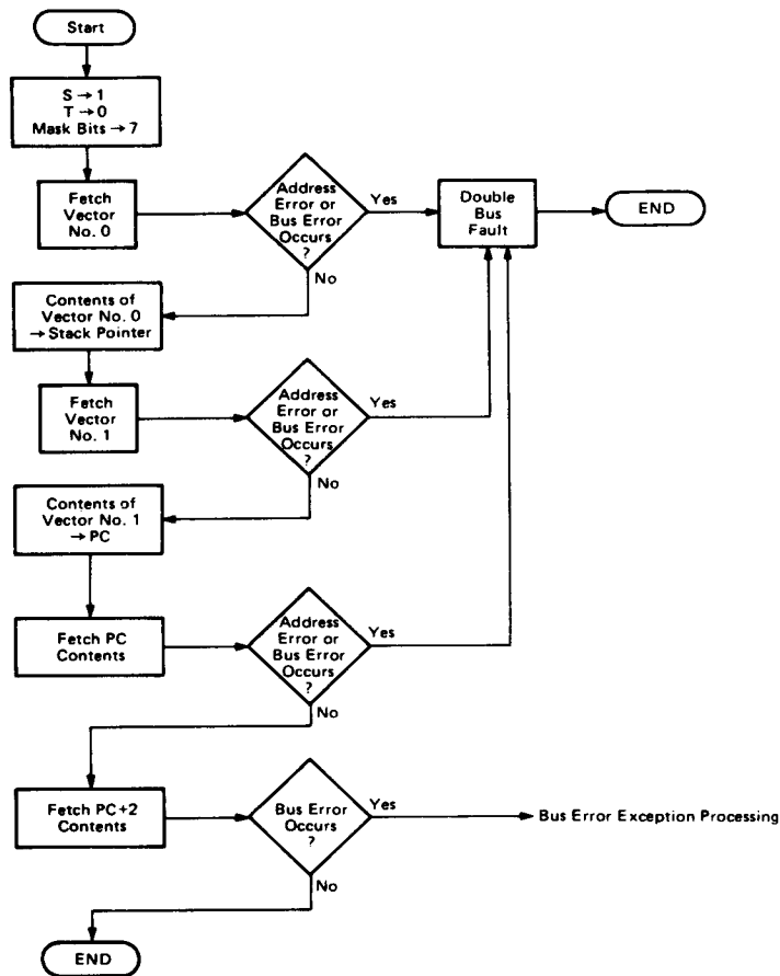
Figure 41 Reset Exception Processing
