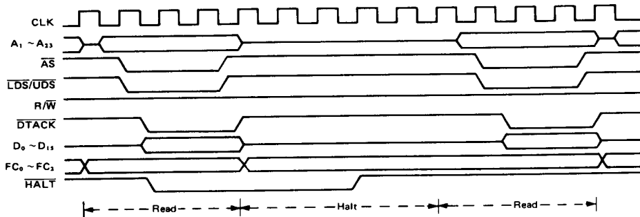
Figure 33 Halt Signal Timing Characteristics
