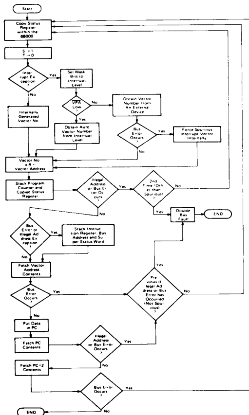
Figure 40 Exception Processing Sequence (Not Reset)
