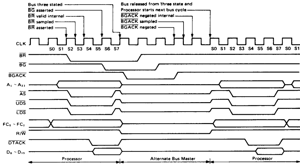
Figure 28 Bus Arbitration During Processor Bus Cycle
