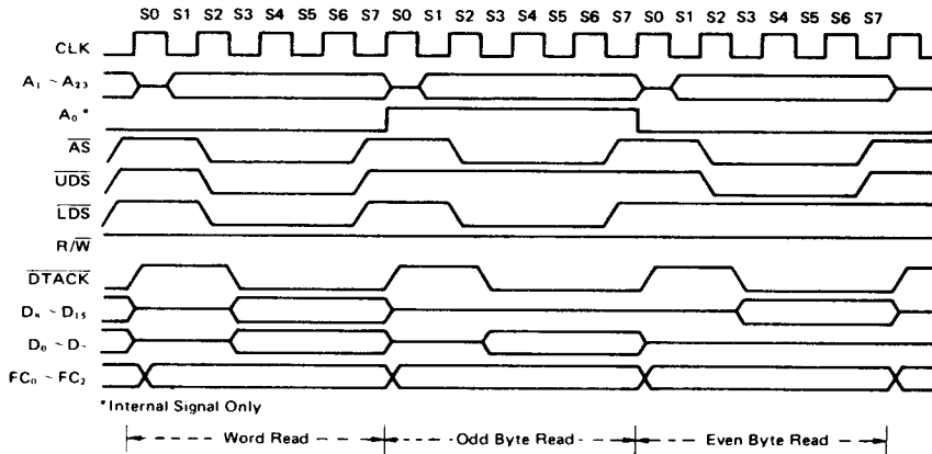
Figure 18 Word and Byte Read Cycle Timing Diagram
