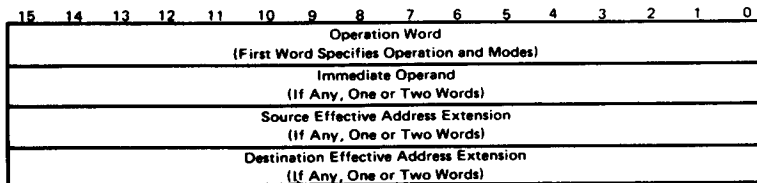
Figure 12 Instruction Format
