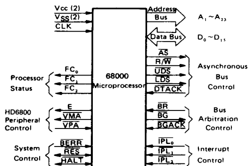
Figure 14 Input and Output Signals
