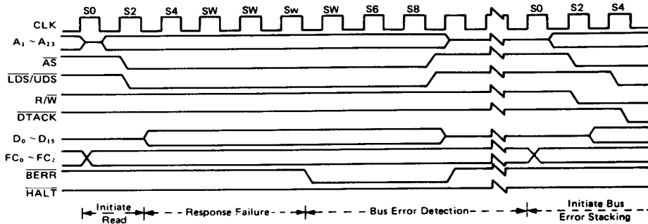
Figure 31 Bus Error Timing Diagram
