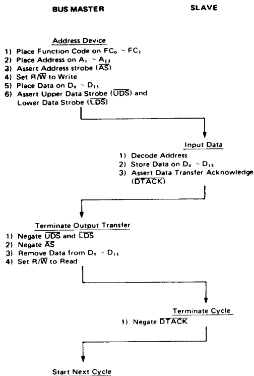
Figure 19 Word Write Cycle Flow Chart
