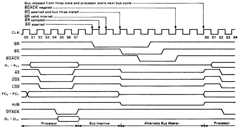
Figure 29 Bus Arbitration with Bus Inactive
