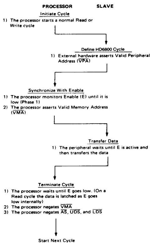
Figure 48 HD6800 Interface Flow Chart
