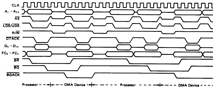
Figure 25 Bus Arbitration Cycle Timing Diagram
