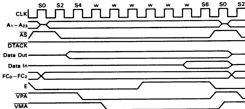
Figure 49 68000 to HD6800 Peripheral Timing—Best Case
