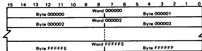
Figure 10 Word Organization in Memory
