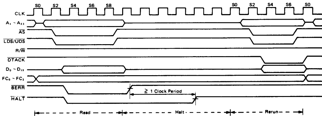
Figure 32 Re-Run Bus Cycle Timing Information
