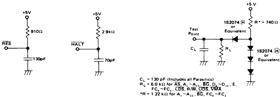
Figure 1 Test Loads
