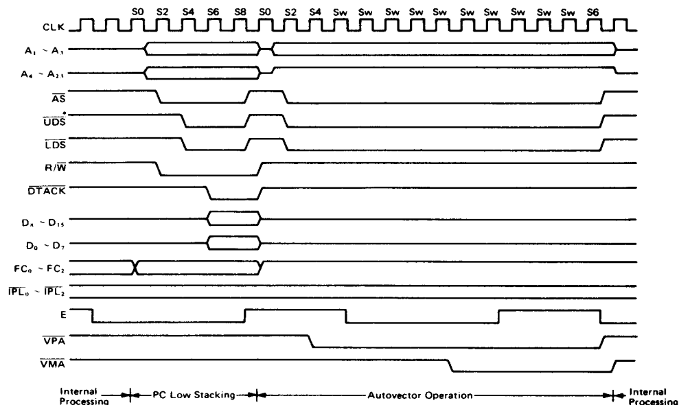
Figure 54 Autovector Operation Timing Diagram
