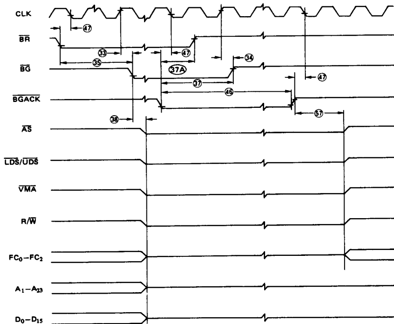
Figure 7. Bus Arbitration Timing Diagram — Idle Bus Case
