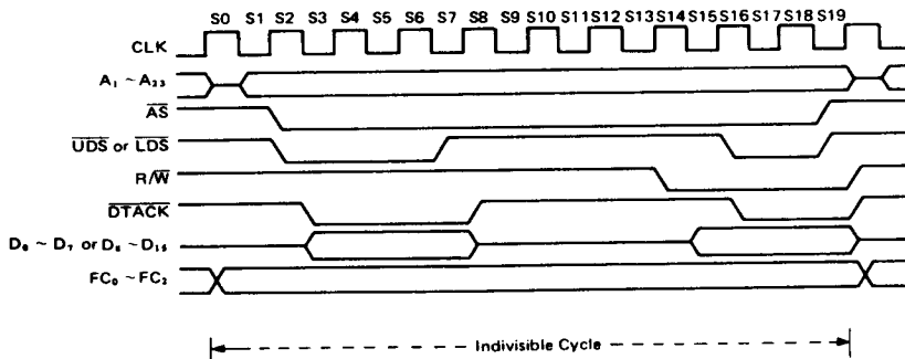
Figure 23 Read-Modify-Write Cycle Timing Diagram
