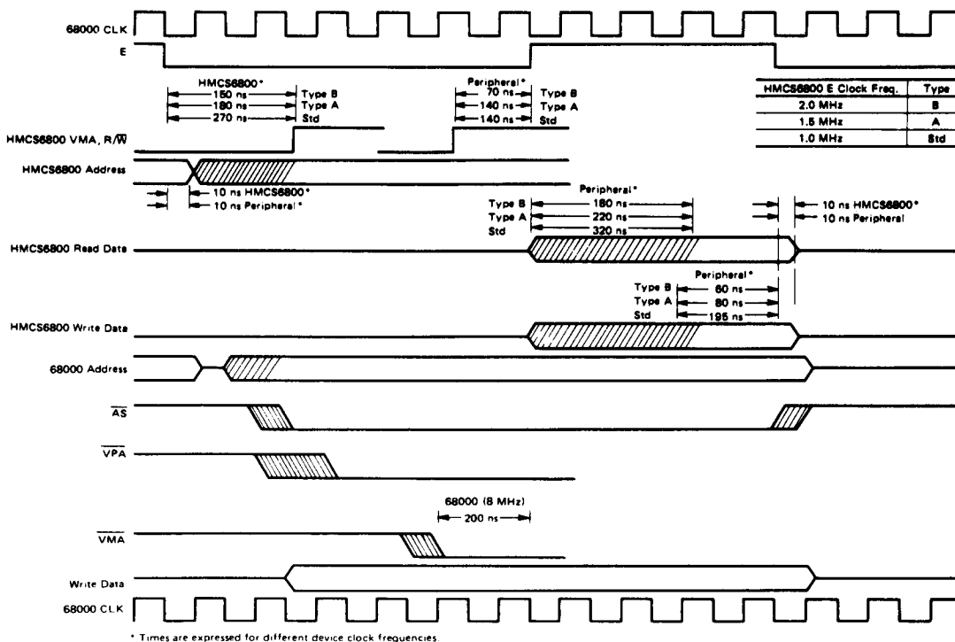
Figure 51 68000 to HD6800 Peripheral Timing Diagram
