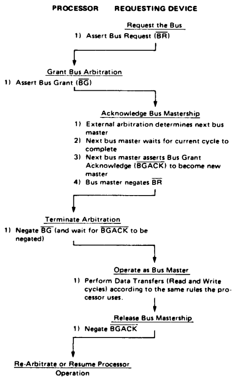
Figure 24 Bus Arbitration Cycle Flow Chart
