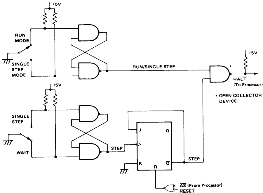
Figure 34 Simplified Single-Step Circuit
