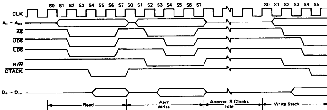
Figure 46 Address Error Timing
