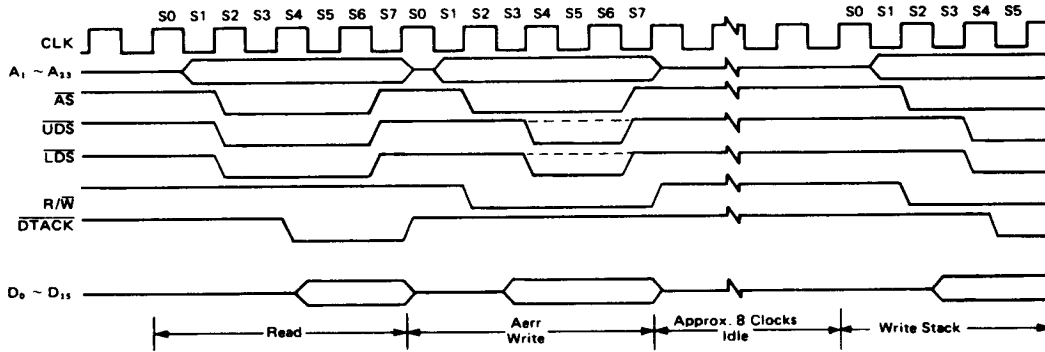
Figure 59 Address Error Timing
