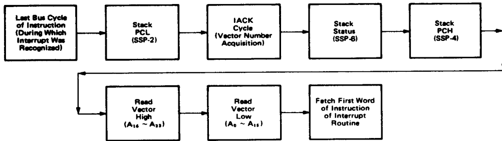
Figure 44 Interrupt Exception Timing Sequence
