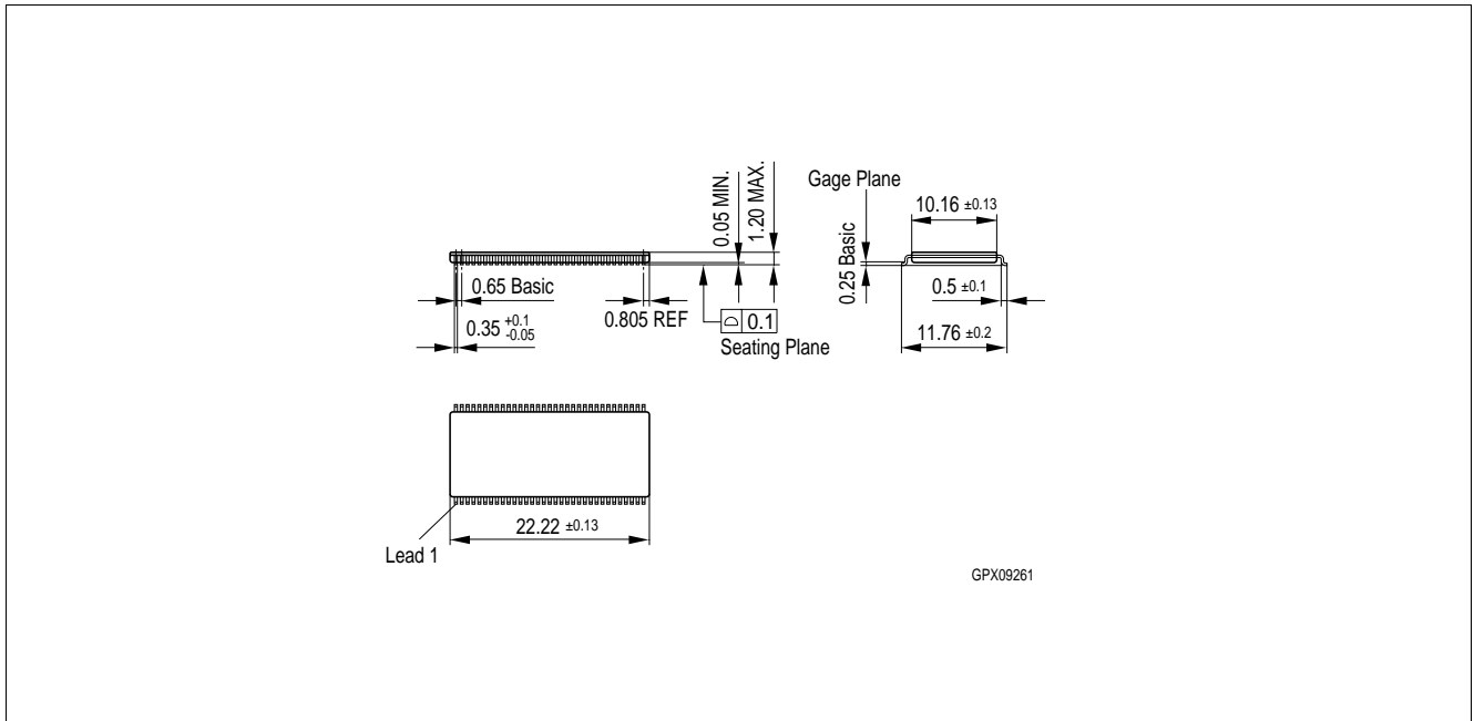
Figure 55 Package Outline of P-TSOPII-66-1 (non-green/green)
