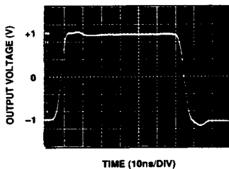
Small Signal Pulse Response
