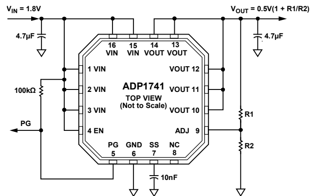
Figure 2. ADP1741 with Adjustable Output Voltage, 0.75 V to 3.0 V
