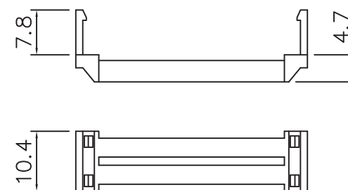
Strain Relief
