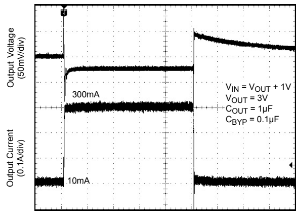
Time (20µs/div)
