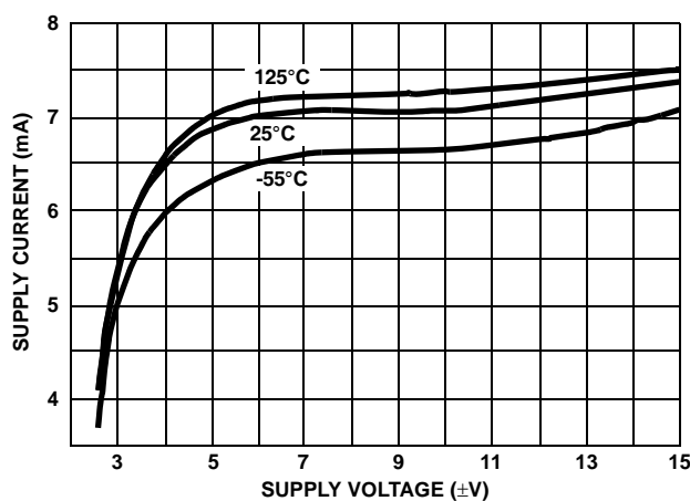
FIGURE 14. SUPPLY CURRENT vs SUPPLY VOLTAGE (AVERAGE OF 30 UNITS FROM 3 LOTS)
