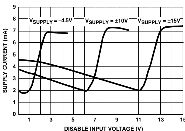
FIGURE 16. SUPPLY CURRENT vs \overline{DISABLE} INPUT VOLTAGE
