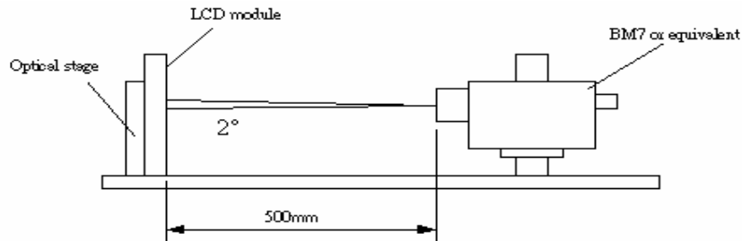
FIG.1 Measurement equipment
