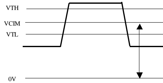
Figure 2 : LVDS Differential Voltage
