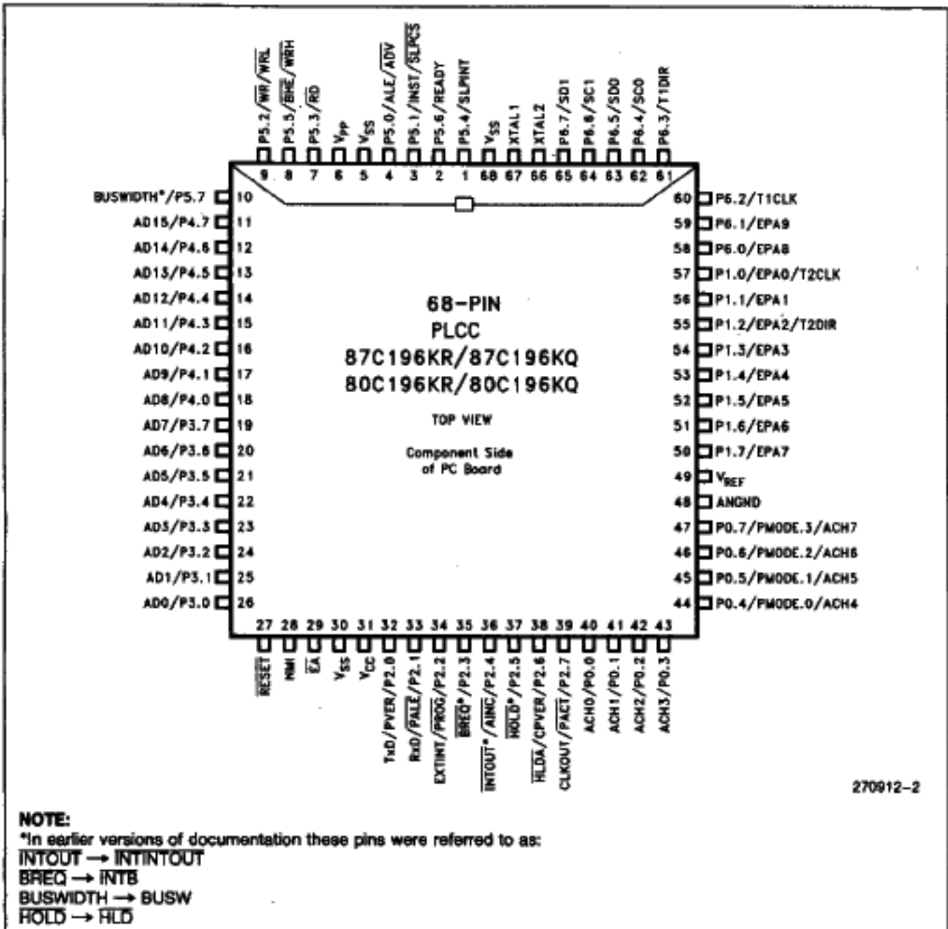
Figure 2. Package Diagrams
