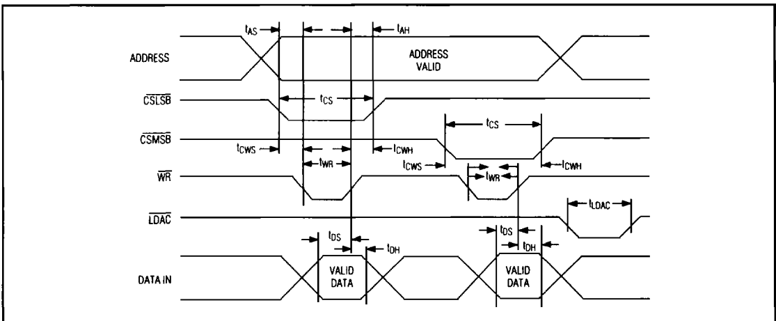
Figure 3. Write-Cycle Timing
