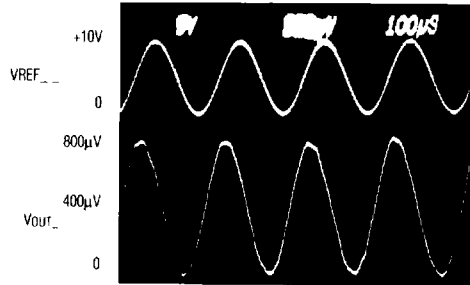
MAX526 REFERENCE FEEDTHROUGH AT 4000Hz
