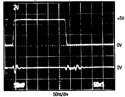
MAX527 DIGITAL FEEDTHROUGH (GLITCH IMPULSE)
