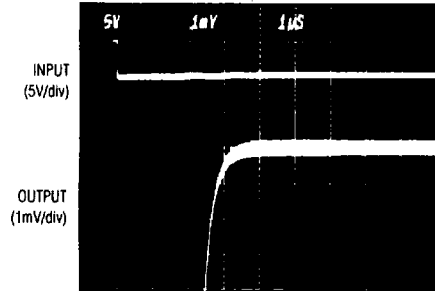
MAX526 NEGATIVE SETTLING TIME TO FULL-SCALE STEP - ALL BITS ON TO ALL BITS OFF
