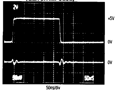
MAX526 DIGITAL FEEDTHROUGH (GLITCH IMPULSE)
