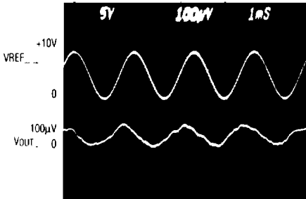
MAX526 REFERENCE FEEDTHROUGH AT 400Hz
