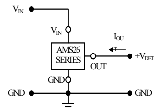
Output Current Test Circuit
