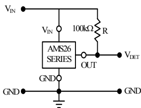
Detector Threshold Test Circuit
