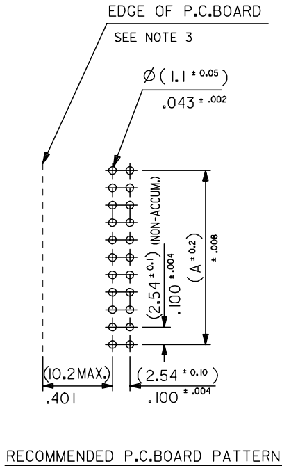
RECOMMENDED P.C. BOARD PATTERN
