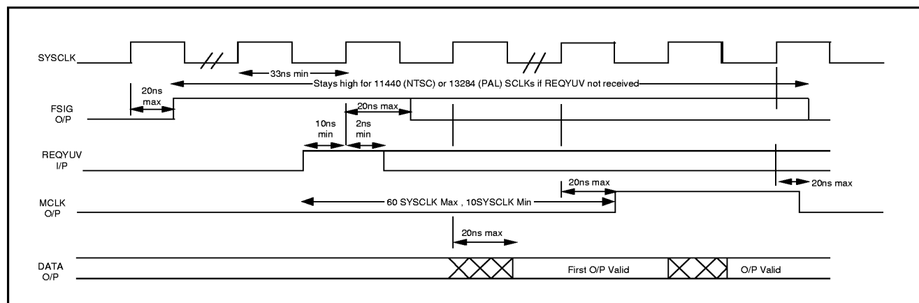
Fig 3 : Macroblock Output Timing
