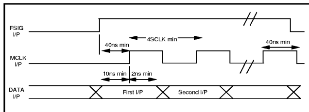
Fig 4 : Macroblock Input Timing
