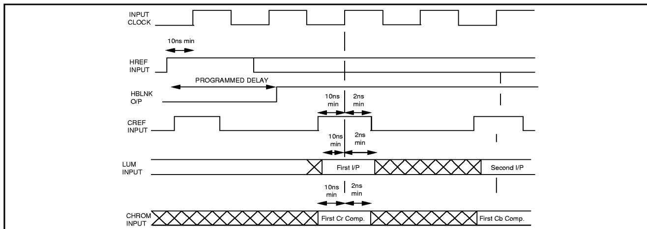
Fig 2 : Luminance and chrominance inputs in the decimate mode.
