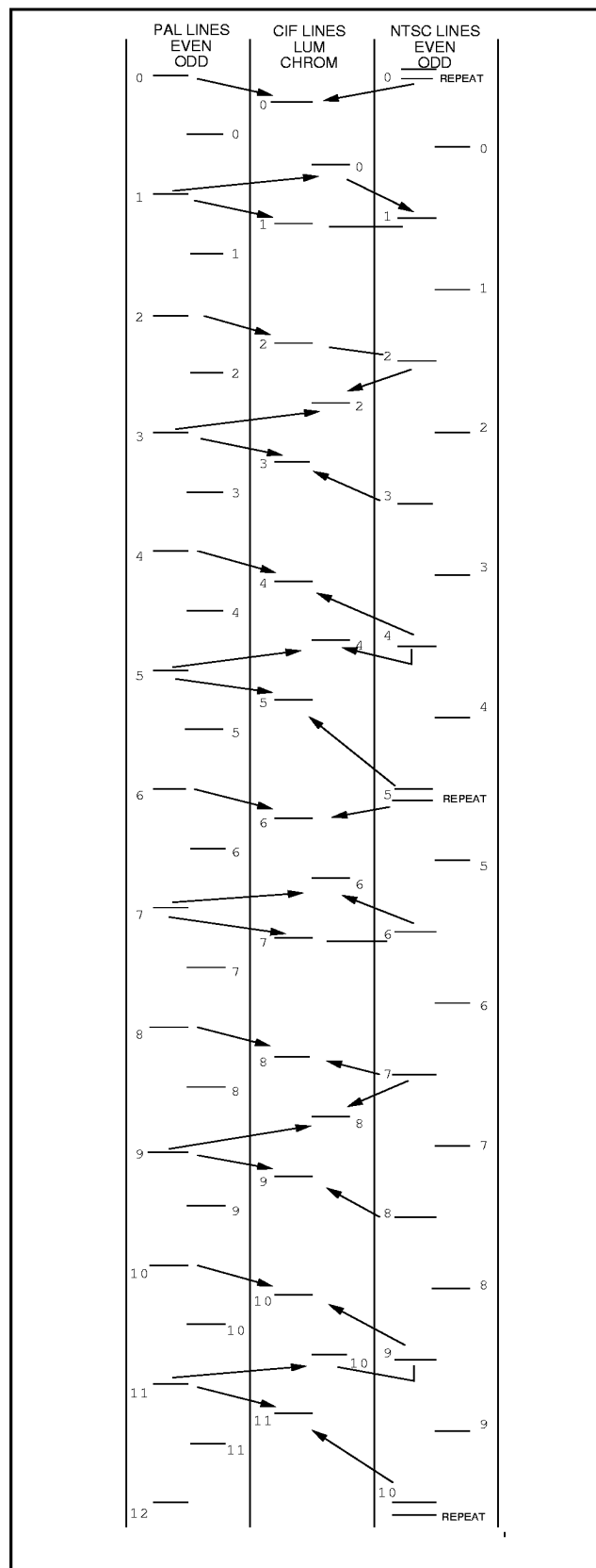
Fig 7 : CIF Spatial Relationships
