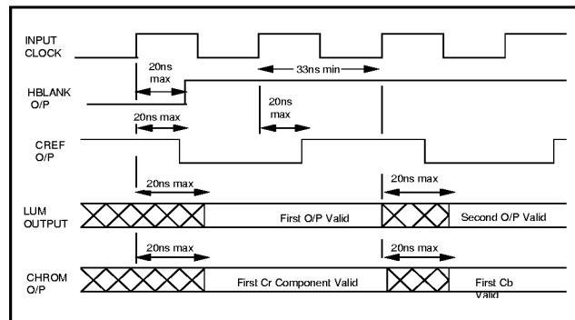
Fig 5 : Luminance and Chrominance Output Timing
