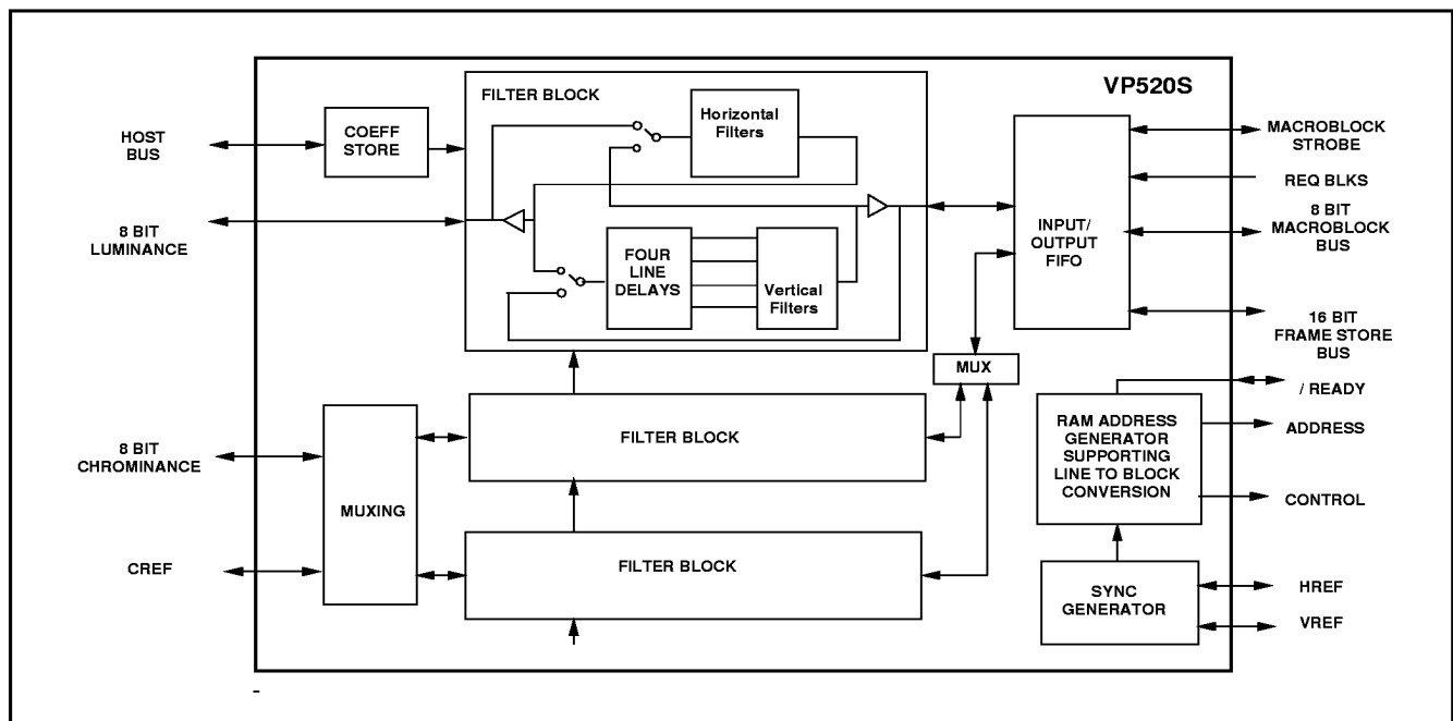
Fig 1 : Simplified Block Diagram
