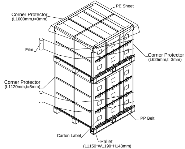
Figure. 8-2 Packing method
