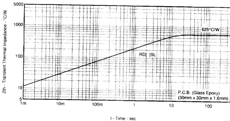
Fig.7 TRANSIENT THERMAL IMPEDANCE CHARACTERISTIC
