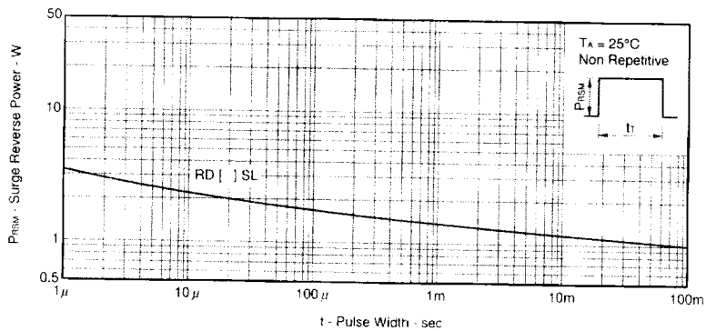
Fig.8 SURGE REVERSE POWER RATINGS
