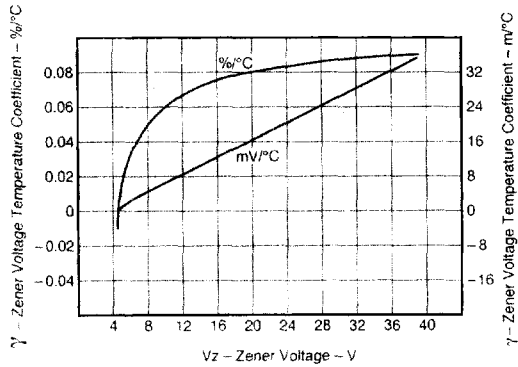
Fig. 6 ZENER VOLTAGE TEMPERATURE COEFFICIENT vs. ZENER VOLTAGE
