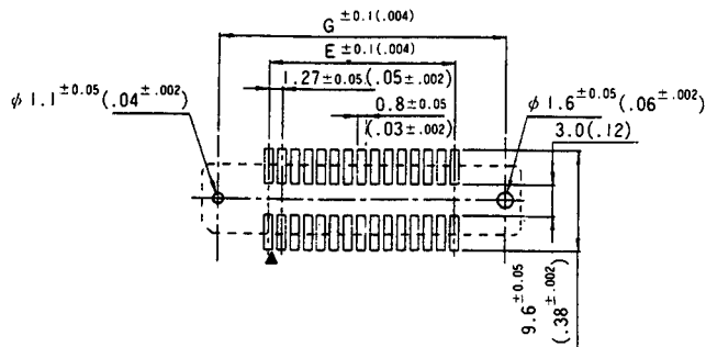
Printed Circuit Board Layout (component side view)
