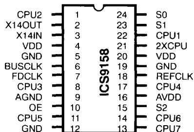
24-Pin PDIP or SOIC J-5, J-7
