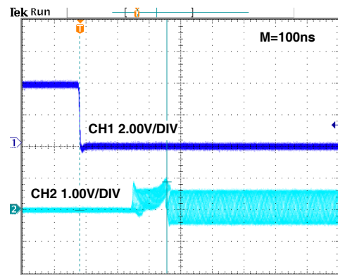
FIGURE 18. ENABLED RESPONSE
