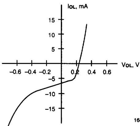
Output, LOW
