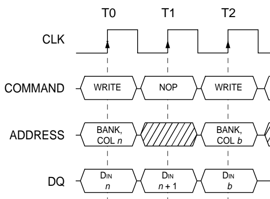
Figure 14 WRITE BURST
