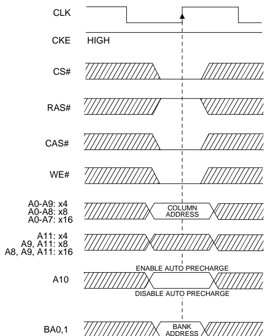
Figure 13 WRITE COMMAND
