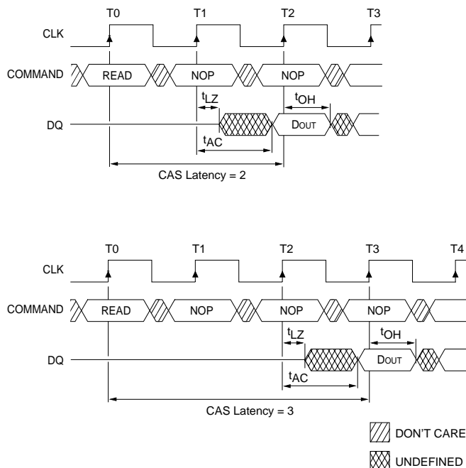
Figure 6 CAS LATENCY
