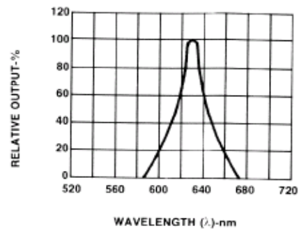
Fig.2 SPECTRAL RESPONSE
