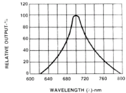
Fig.2 SPECTRAL RESPONSE
