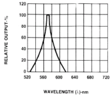
Fig.2 SPECTRAL RESPONSE
