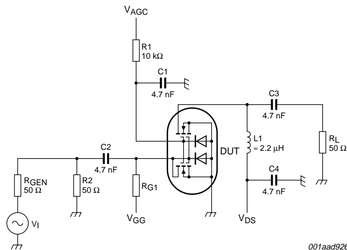
Fig 32. Cross-modulation test setup (for one MOSFET)
