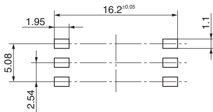
PCB layout for reference only
