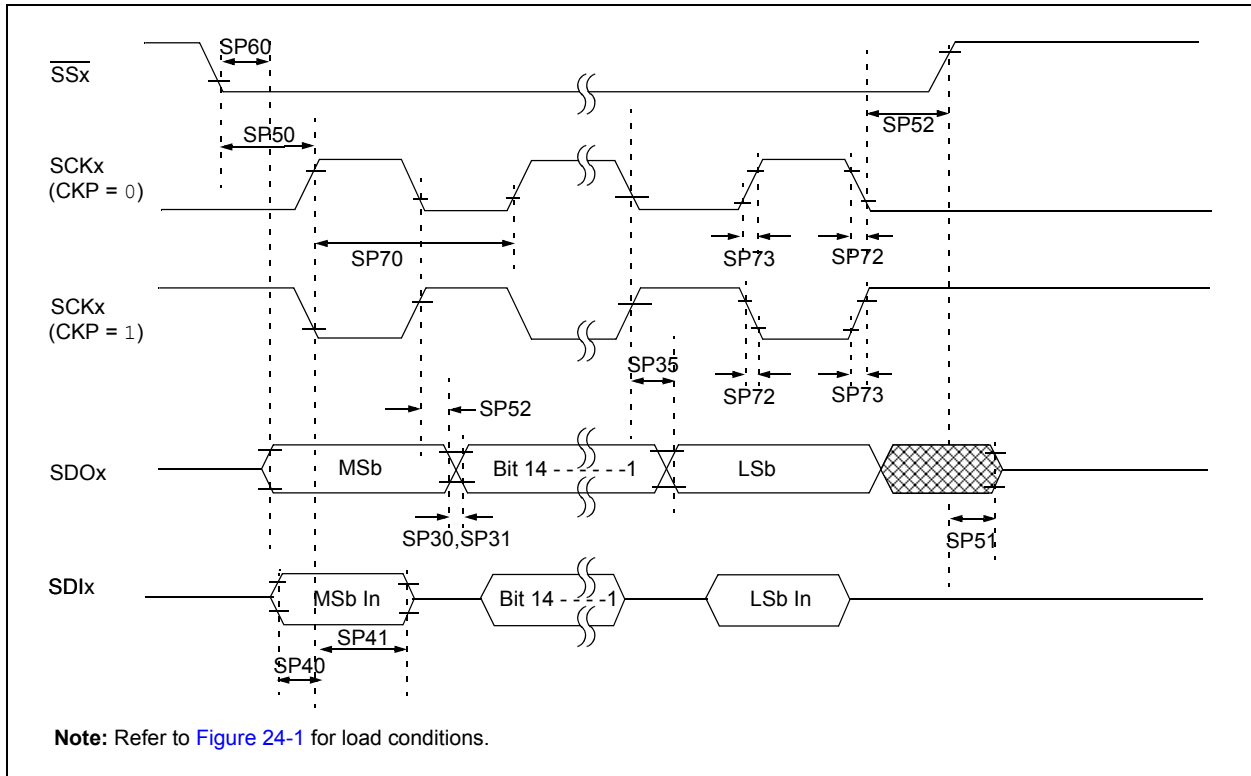
FIGURE 24-14: SPIx SLAVE MODE (FULL-DUPLEX, CKE = 1, CKP = 1, SMP = 0) TIMING CHARACTERISTICS
