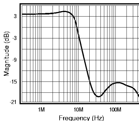
Figure 11: Lowpass Response
