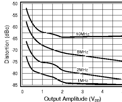
3rd Harmonic Distortion, R_L = 1\text{ k}\Omega
