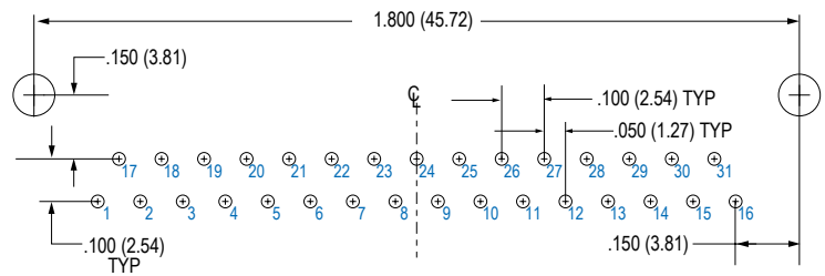
31 SOCKET MWDM-31SBR
