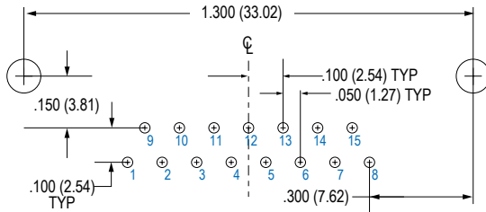
15 SOCKET MWDM-15SBR
