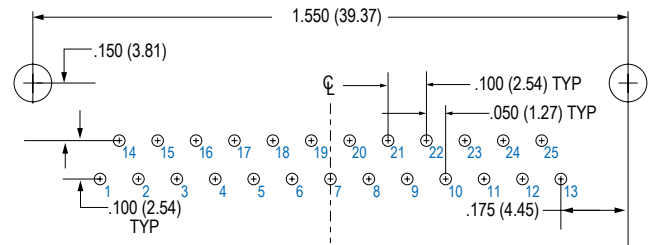
25 SOCKET MWDM-25SBR
