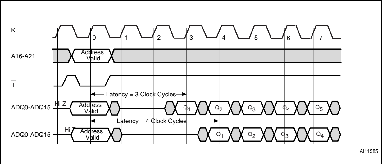
Figure 3. Variable Latency Mode, No Refresh Collision
