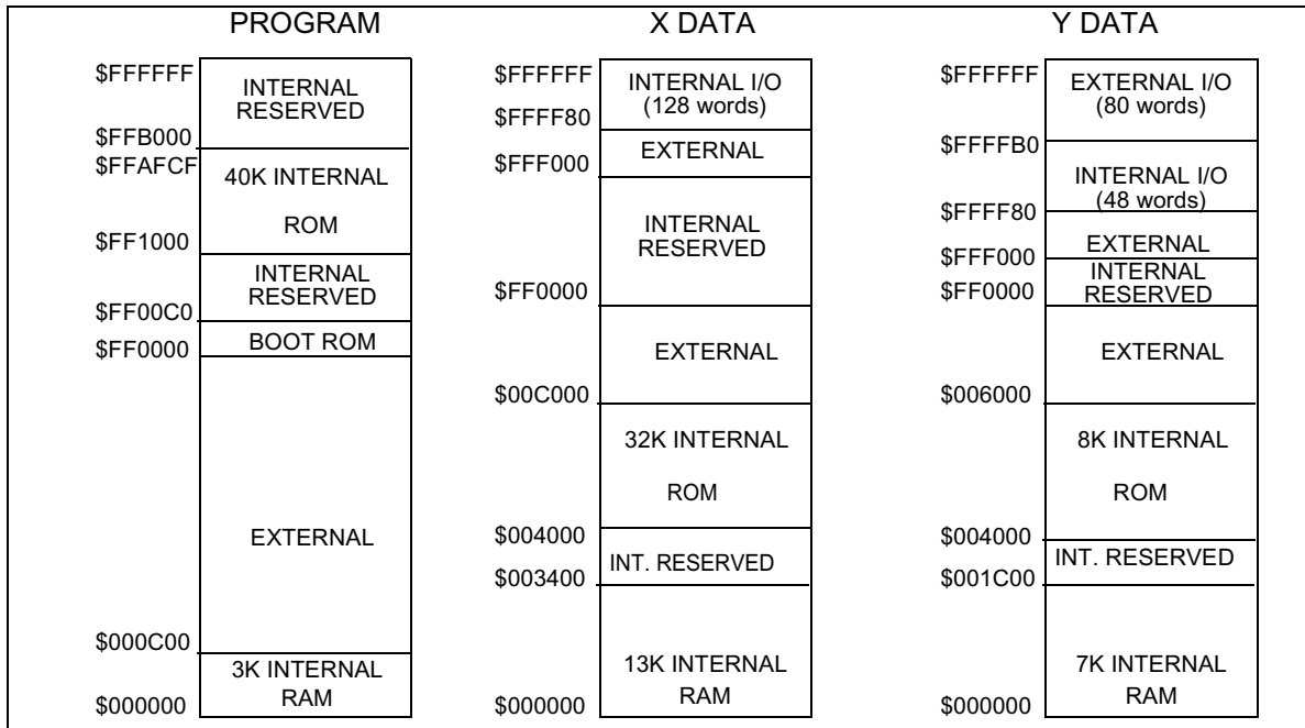
Figure 5-1 Memory Maps for MSW=(X,X), CE=0, MS=0, SC=0
