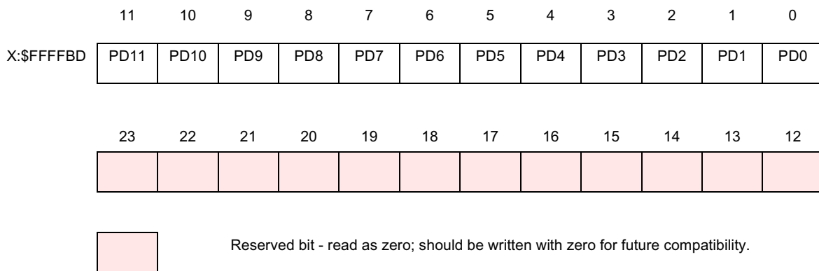
Figure 10-21 PDRC Register
