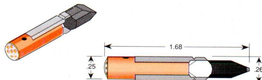
Series: 68SB206 (6 Chip 160° Illumination) PN Example: 68SB206-0UO-120A
