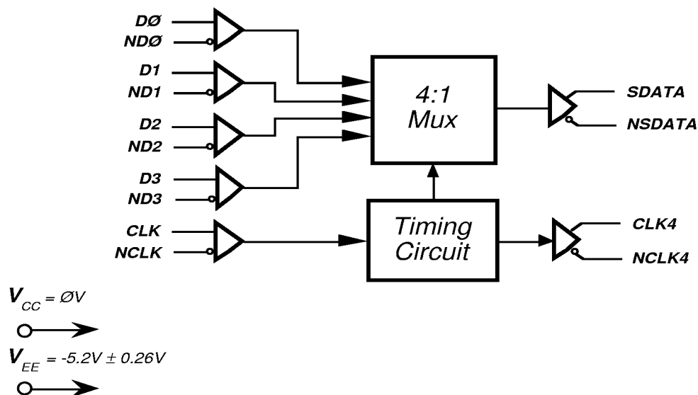
Figure 2: VS8005 Block Diagram
