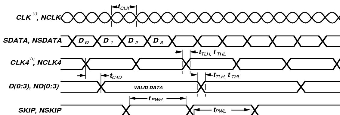
Figure 4: VS8005 Waveforms
