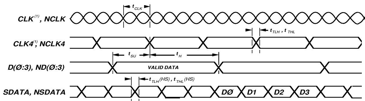
Figure 3: VS8004 Waveforms
