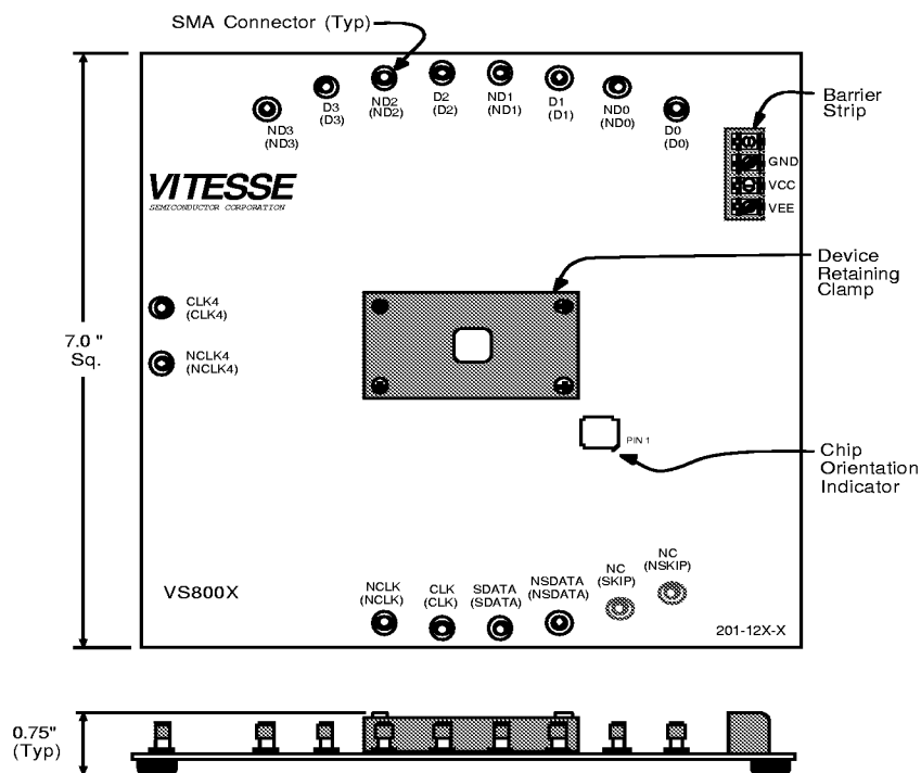
Figure 8: VS8004/VS8005 DUT Boards
