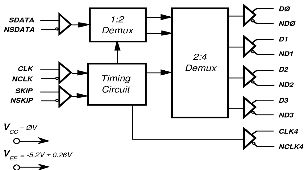
Figure 2: VS8005 Block Diagram
