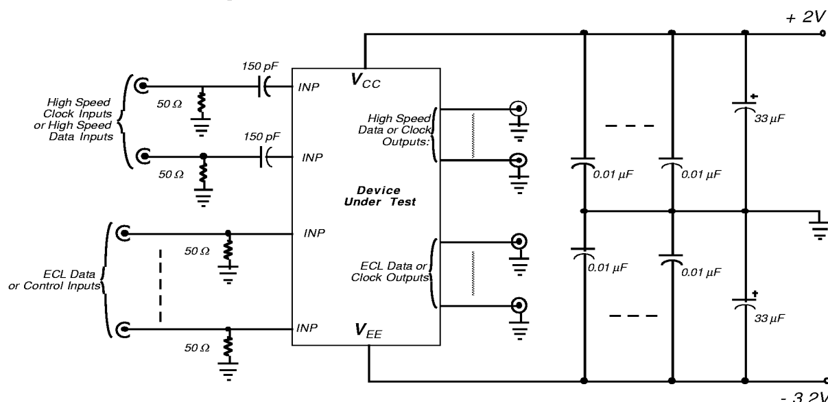
Figure 7: VS8004/VS8005 DUT Board Schematics
