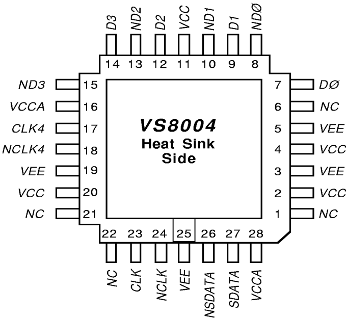
Figure 5: VS8004 Pin Diagram
