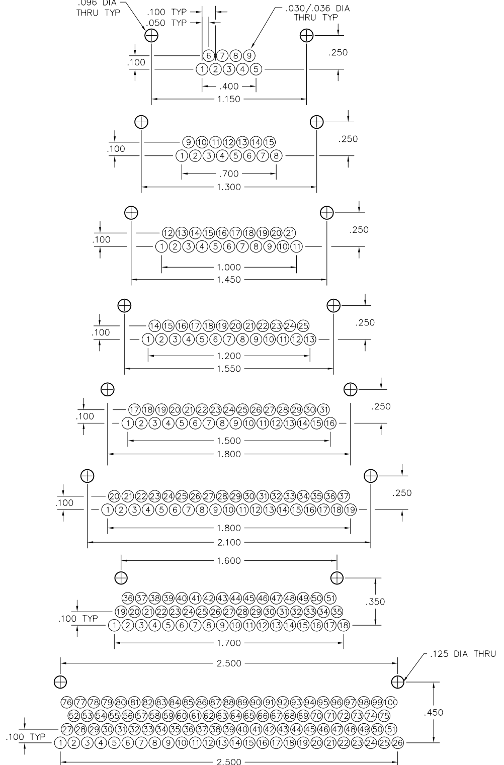
RECEPTACLE PC BOARD LAYOUT COMPONENT SIDE
